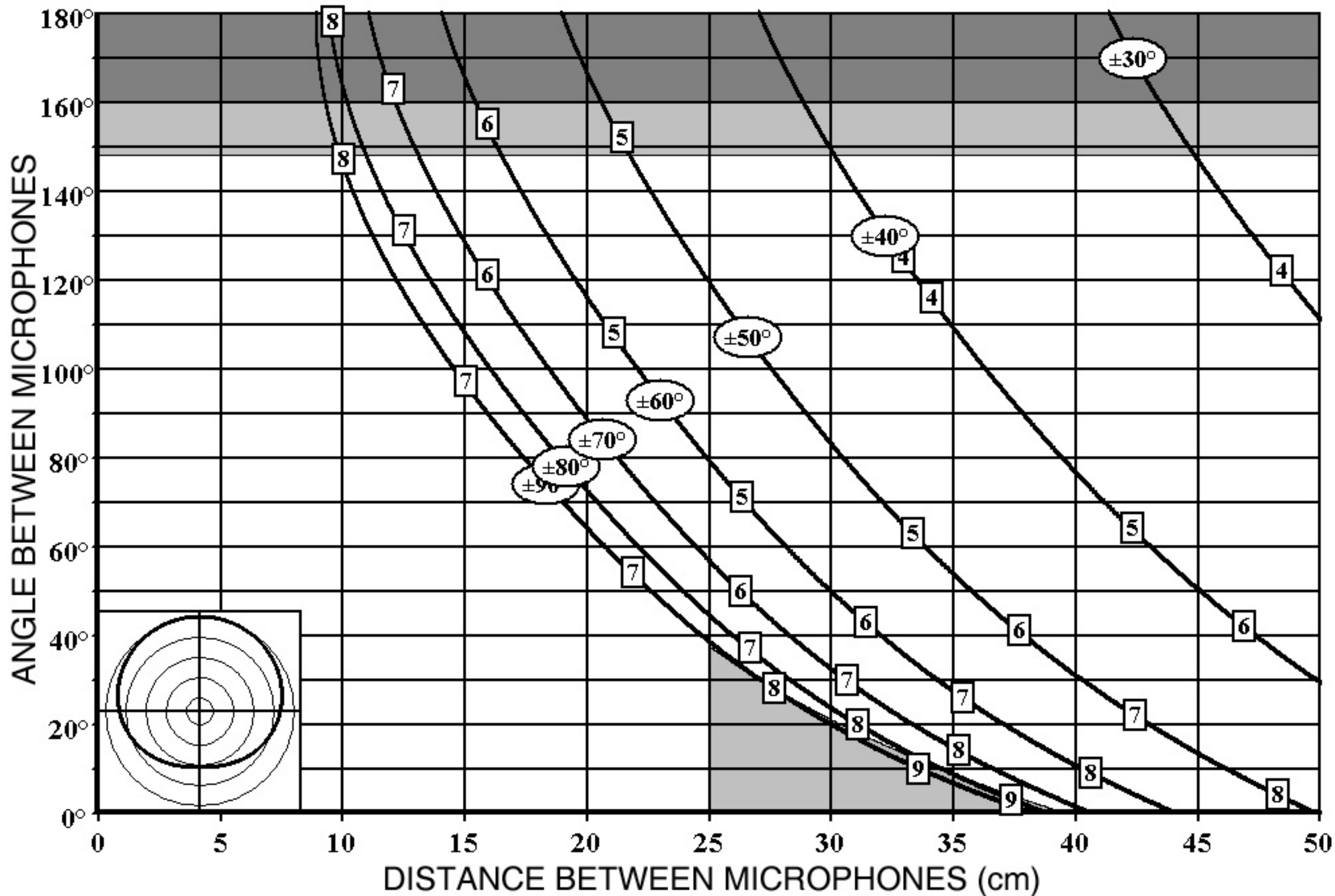
SRA Diagram for Hypocardioid Microphone (back attenuation 10dB)
