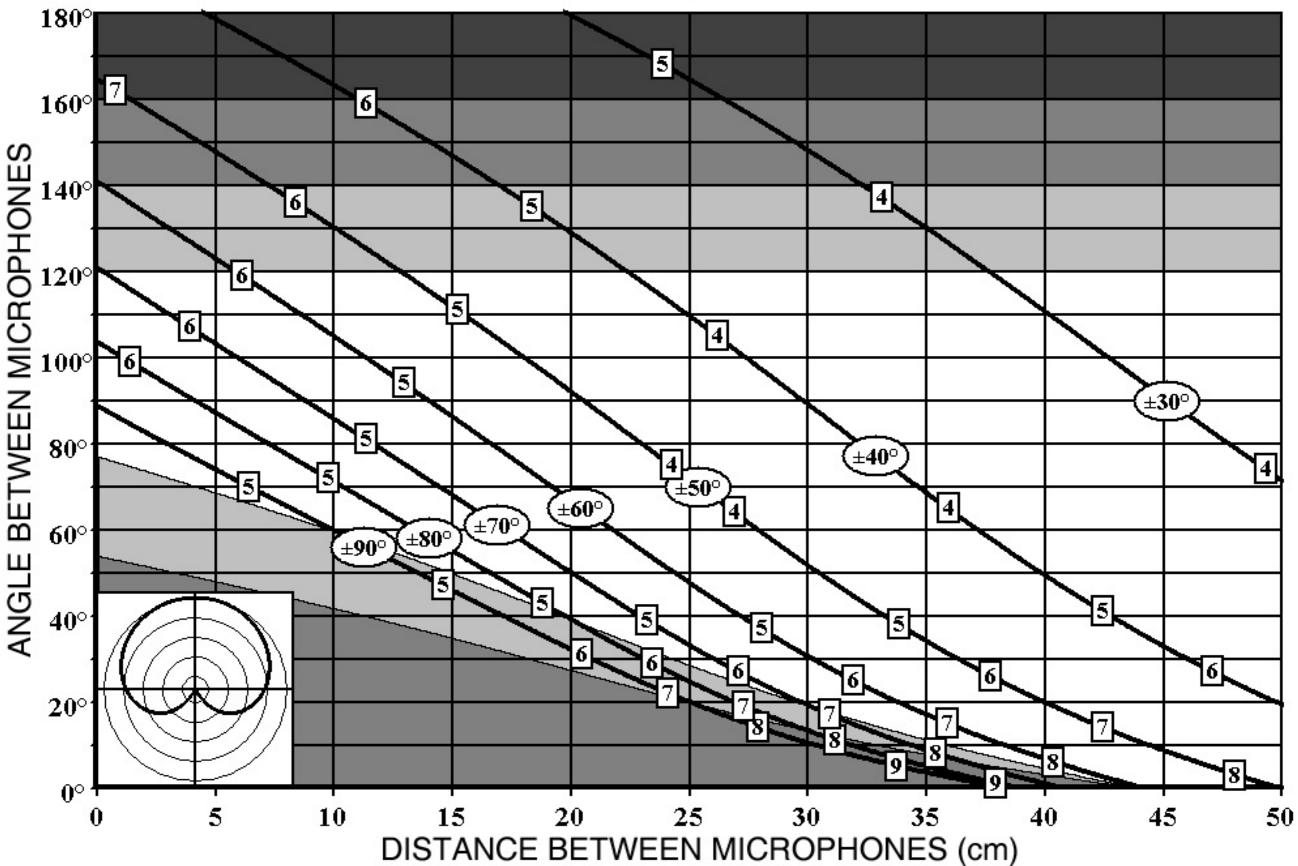
SRA Diagram for Cardioid Microphones (6db attenuation at 90°)
